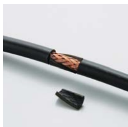
Insulation removal
